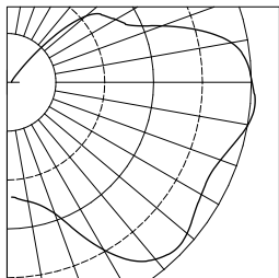
BIS175MXX-BRI-GEP TEST NUMBER: 26258P LAMP: 175W MH, COATED LUMENS: 15,000 MOUNTING HEIGHT: 12 FEET
