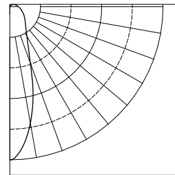
BIS18WLXX-BRI-GE5 TEST NUMBER: 27585 LAMP: 18W LED NEUTRAL WHITE LUMENS: 700 MOUNTING HEIGHT: 12 FEET
