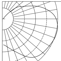
BIS42CCXX-BRI-GEP TEST NUMBER: 26277P LAMP: 42W CFL LUMENS: 3,200 MOUNTING HEIGHT: 12 FEET
